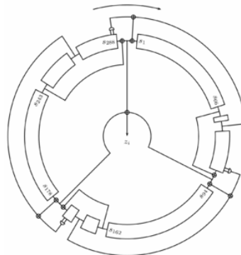
Fig.3: Trivium algorithm
