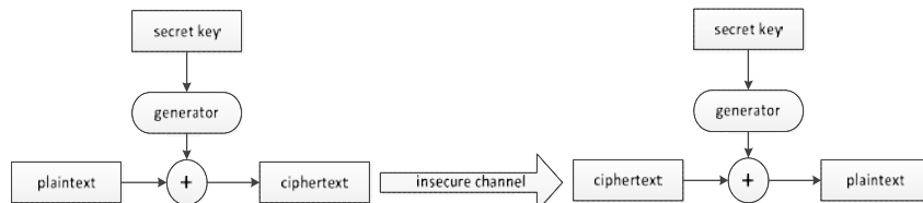
Fig.2 Stream Cipher Example
