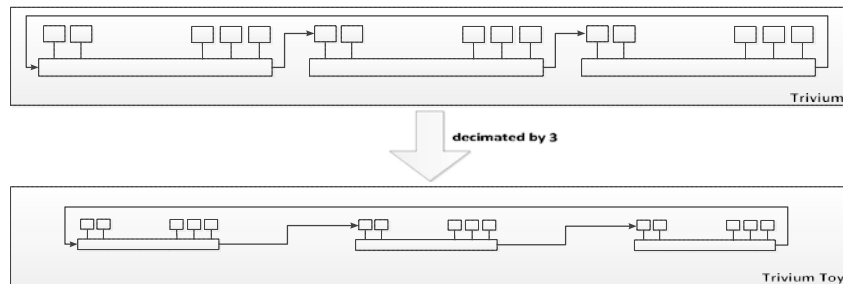
Fig.5 Trivium vs Trivium Toy
