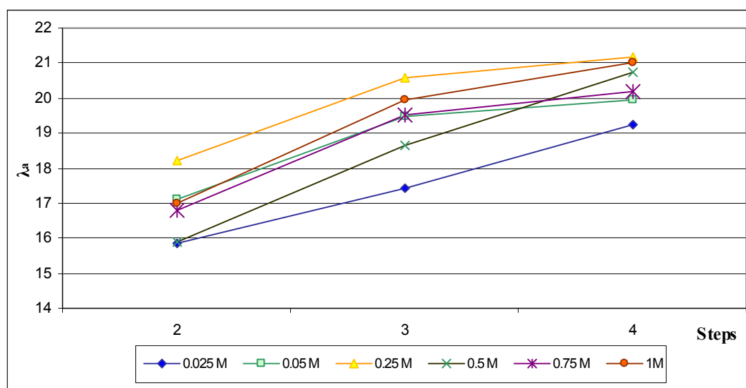
Figure 4. Average number of water molecules per sulfonic acid group obtained for the different steps in the treatment with H 3 PO 4 .
