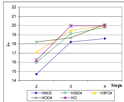
Figure 8. Comparing average number of water molecules per sulfonic acid group obtained with different acids 0.05 M
