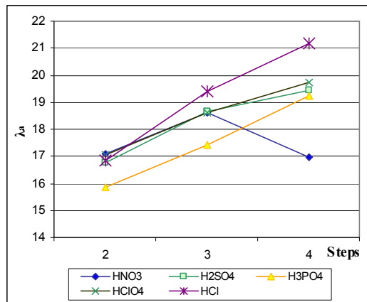
Figure 7. Comparing average number of water molecules per sulfonic acid group obtained with different acids 0.025 M
