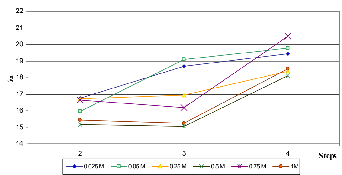
Figure 3. Average number of water molecules per sulfonic acid group obtained for the different steps in the treatment with H 2 SO 4 .
